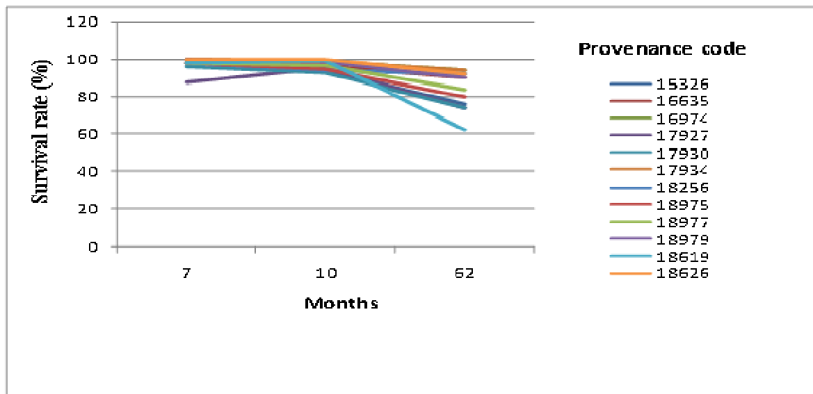
Figure 3: Survival (%) trends of those planted Acacia mearnsii provenances.
