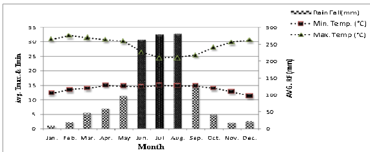
Figure 2:-Mean monthly rainfall (RF), maximum and minimum temperature (Temp.) of the study area during the five years trial period (2002-2007)
