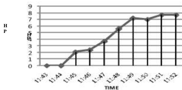
Figure 5. pH versus Time graph in clean water.
