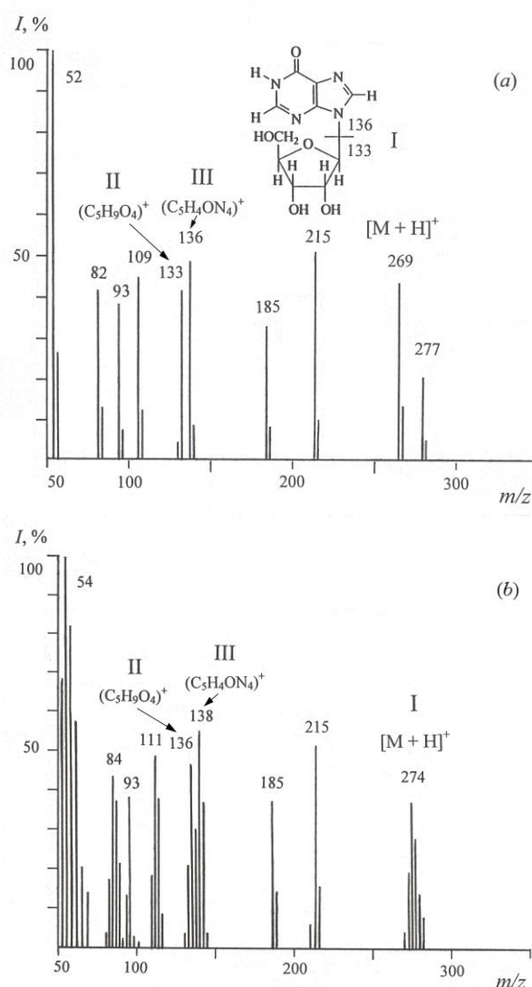
Figure 5: FAB mass spectra of inosine (glycerol as a matrix) under different experimental conditions: (a) – natural inosine; (b) – [^2\text{H}] inosine isolated from HW medium (scanning interval at m/z 50–350; major peaks with a relative intensity of 100% at m/z 52 and m/z 54; ionization conditions: cesium source; accelerating voltage, 5 kV; ion current, 0.6–0.8 mA; resolution, 7500 arbitrary units): I – relative intensity of peaks (%); (I) – inosine; (II) – ribose fragment; (III) – hypoxanthine fragment.
