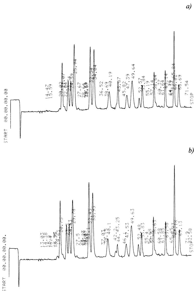
Figure 12: Ion exchange chromatograms of amino acids obtained from hydrolizates of protonated (a) and deuterated (b) cells of B. subtilis on the maximally deuterated D_2O -medium: Biotronic LC-5001 (230×3.2 mm) column (“Eppendorf–Nethleler–Hinz”, Germany); stationary phase: UR-30 sulfonated styrene resin (“Beckman–Spinco”, USA); 25 \mu m ; 50–60 atm; mobile phase: 0.2 N sodium–citrate buffer (pH = 2.5); the eluent input rate: 18.5 ml/h; the ninhydrin input rate: 9.25 ml/h; detection at \lambda = 570 and \lambda = 440 nm (for proline).
