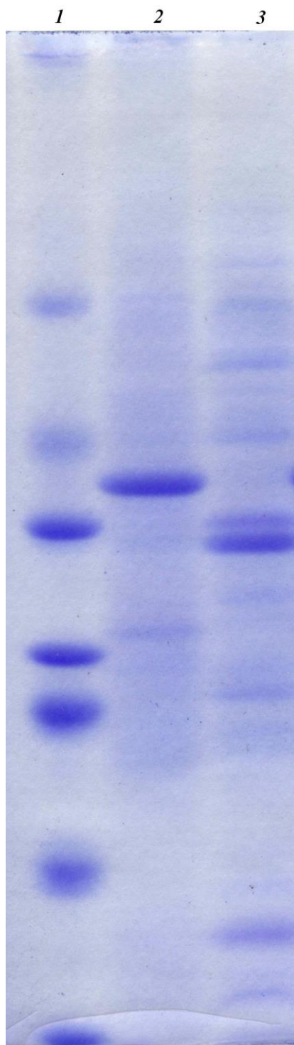
Figure 14: Electropherograms of proteins isolated from hydrolysates of total biomass of B. subtilis : 1 – a standard set of proteins; 2 – a sample obtained from protonated medium; 3 – a sample obtained from D 2 O-medium
