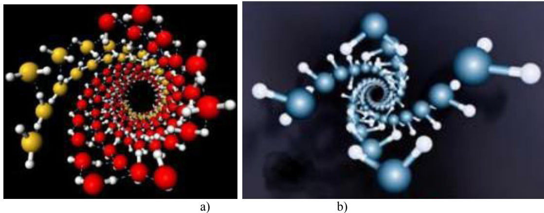
Figure 3. Structures of water crystals in carbon nanotubes according to computer simulations (Bai et al. , 2006) (diameter of nanotubes 1.35–1.90 nm; pressure 10–40000 atm; temperature -23^0\text{C} ): a) – a general view of the crystal structure of water in nanotubes, b) – the inner wall of the structure of water.
