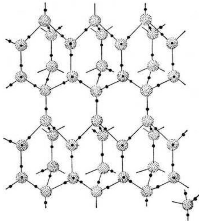
Figure 2. Hydrogen bonding in crystalline structure of natural ice I_h under the temperature -10^0\text{C} and pressure 1 atm. Grey balls – oxygen atoms, black balls – hydrogen atoms. On the right below shown the structural unit of crystalline ice structure.
