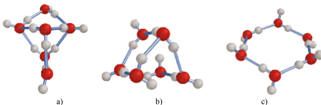
Figure 8. Calculation of small water cluster structures (a-c) with general formula (\text{H}_2\text{O})_n , where n = 6 (Tsai & Jordan, 1993).
