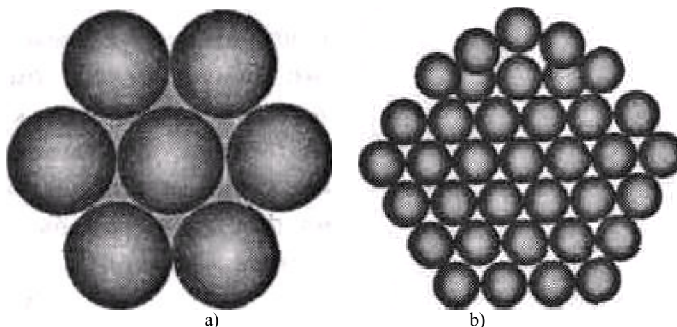
Figure 5. The sphere (a) and the pentagonal (b) packing of balls representing H_2O molecules in clusters. In 1957 S.Frank and W. Wen proposed a model, postulating arbitrary formation of cyclic associates in water, which presumably had random groups of water associates – the “flickering clusters” with general formula (H_2O)_n , which are in a dynamic equilibrium with free H_2O molecules (Henry et al. , 1957). The hydrogen bonds between H_2O molecules are in dynamic equilibrium; they are constantly broken and re-formed in new configurations within a certain time interval; these processes are occurred cooperatively within short-living associated groups of H_2O molecules (clusters), which life spans are estimated from 10^{-10} to 10^{-11} sec. Water associates evidently may have polymer structure, because hydrogen bond is on 10% partially covalent
