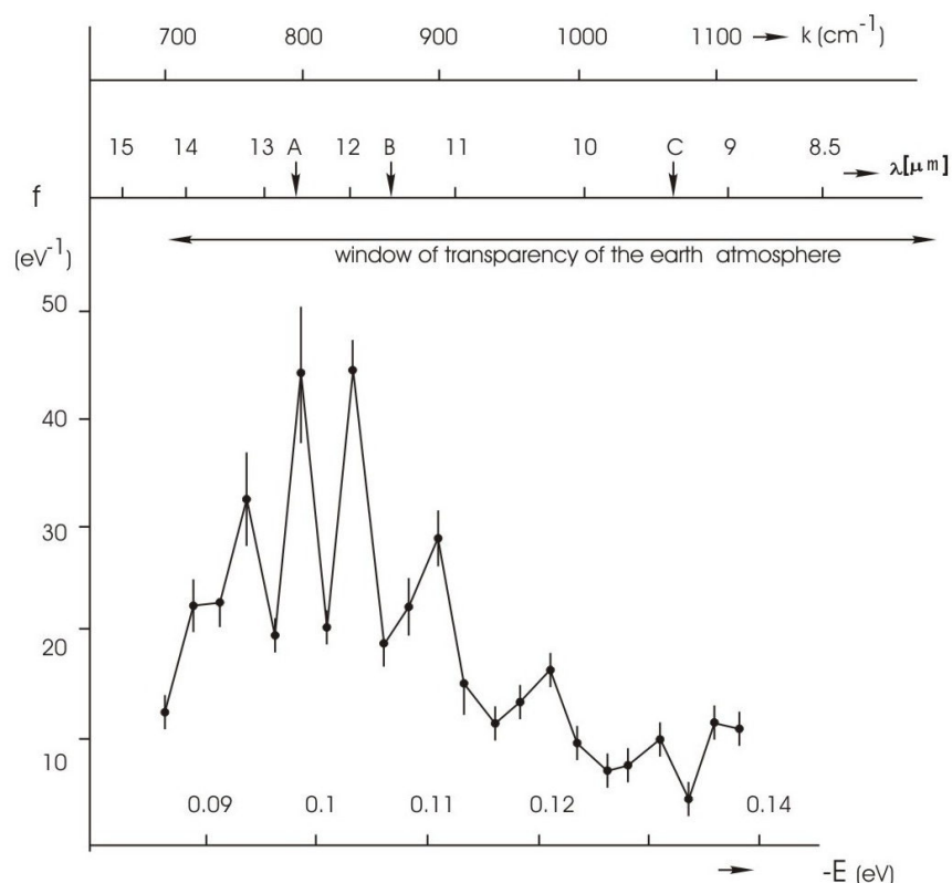
Figure 7. DNES-spectrum of deionized water (chemical purity 99.99%, pH = 6.5–7.5, total mineralization 200 mg/l, electric conductivity 10 \mu\text{S/cm} ). On the horizontal axis shows the energy of the H...O hydrogen bonds in the associates -E (eV). The vertical axis – energy distribution function -f ( \text{eV}^{-1} ). k – the vibration frequency of the H–O–H atoms ( \text{cm}^{-1} ); \lambda – wavelength (mm).
